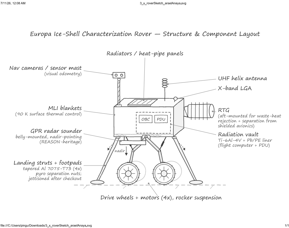
Figure 3: Annotated structural sketch of the rover chassis, deck, radiation vault, antenna mast, and landing-leg arrangement.
